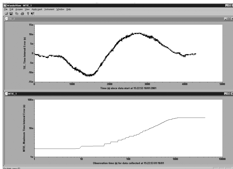
Figure 2: WanderView screen, showing a TIE-curve (top) and a MTIE curve (bottom).
